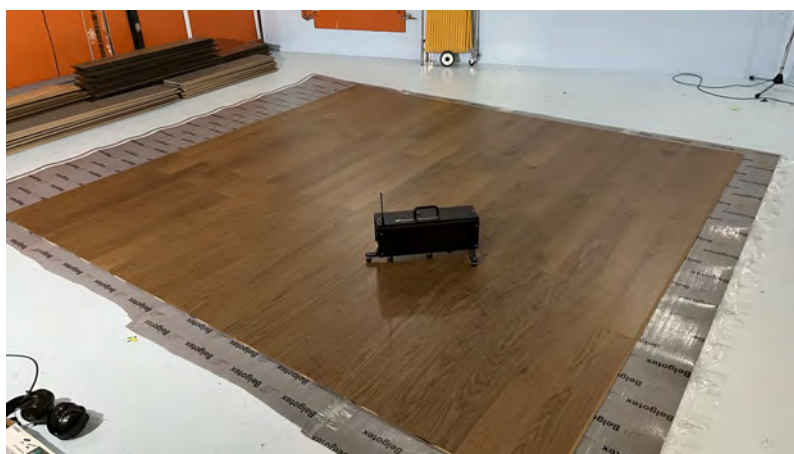
Figure 2.2: Bjelin 9.2mm finished floor system under test
