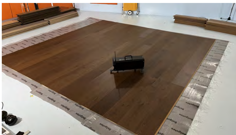
Figure 2.2: Bjelin 11.3mm finished floor system under test
